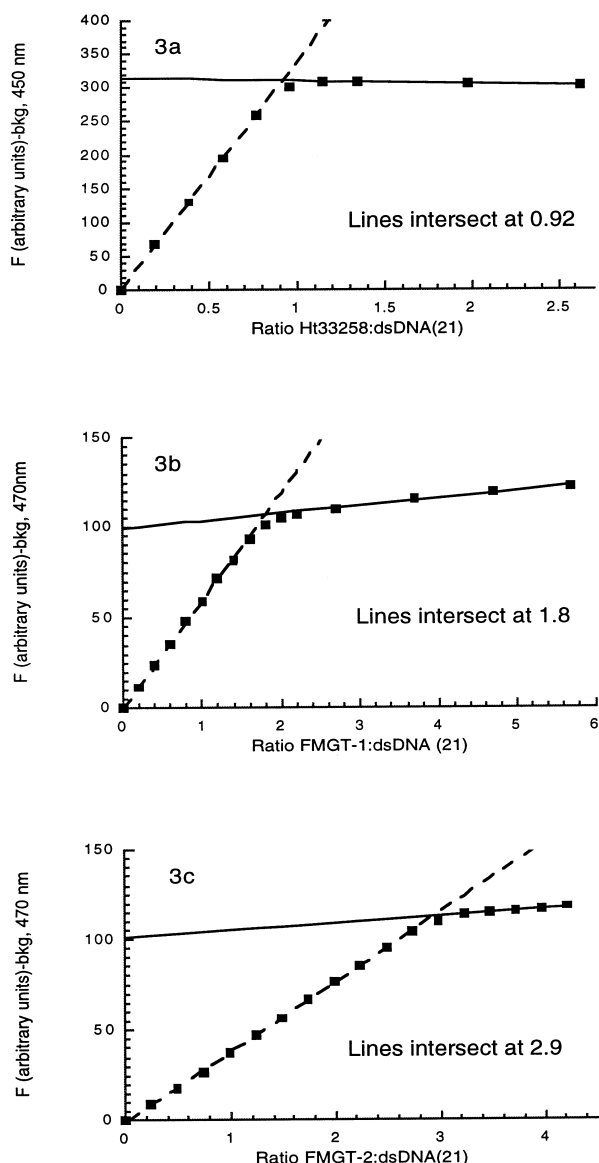
Figure 3. Representative fluorescent titrations of a constant concentration of dsDNA, 50 \mu\text{M} , with ligand for determination of ligand:dsDNA stoichiometries. Samples were excited at 354 nm and their fluorescence emission scanned between 400 and 500 nm. Plots shown are of signal intensity subtracted by background intensity. (a) Titration with Hoechst 33258. (b) Titration with FMGT-1. (c) Titration with FMGT-2.
