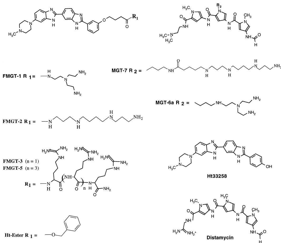
Figure 1. The structures of FMGT-1, -2, -3, and -5, Ht-Ester, tripyrrole peptide MGT-7, and -6a, Hoechst 33258, and distamycin.
