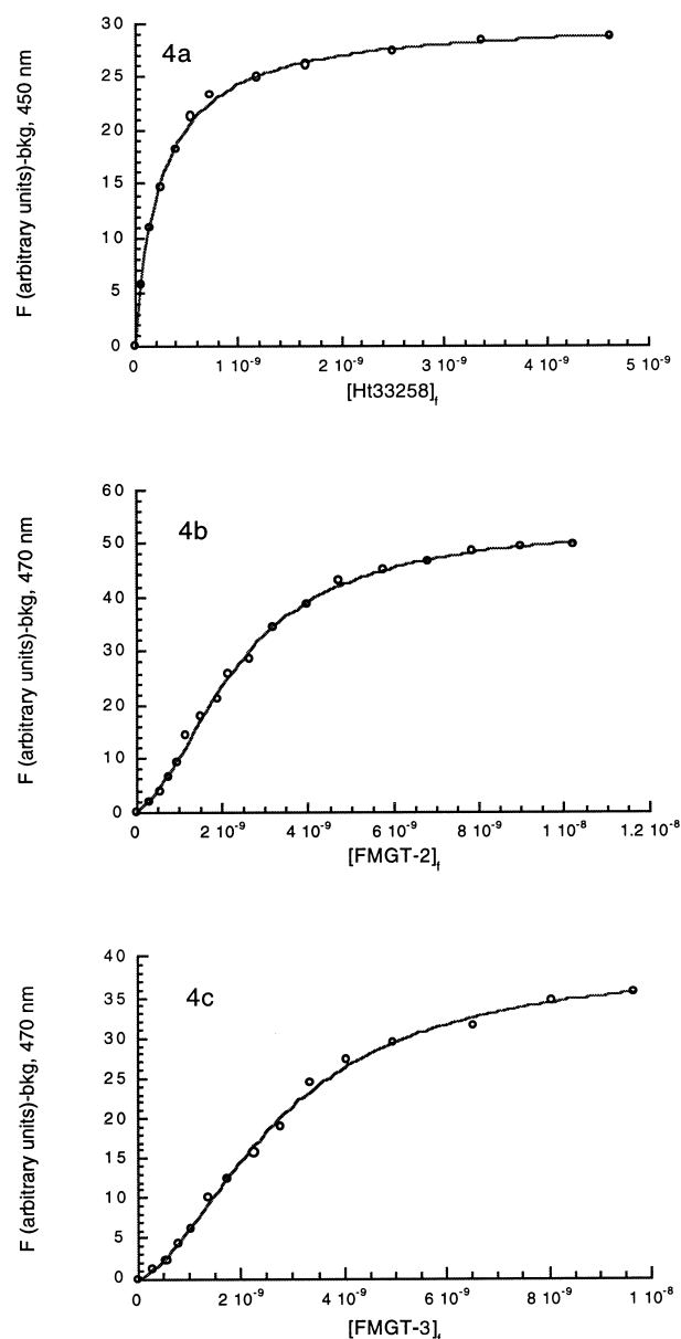
Figure 4. Isothermal binding curves generated by fluorescent titrations of a constant concentration of dsDNA with ligand. Samples, 1–5 nM 21 , were titrated with concentrated ( \mu\text{M} ) ligand solutions. Samples were excited at 354 nm and their fluorescence emission monitored at the appropriate wavelength. Fluorescence intensities have been subtracted by the background value. The x-axis gives the concentration of unbound ligand [L]_f as calculated by eq (4) (see text). Data points are then fit using the theoretical model described by eqs (1), (5), or (6) and a nonlinear least squares curve fitting routine. (a) 1 nM 21 titrated with Hoechst 33258. (b) 2 nM 21 titrated with FMGT-2. (c) 1 nM 21 titrated with FMGT-3.
