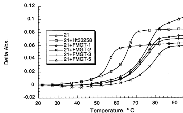
Figure 2. Thermal melting curves for dsDNA:ligand complexes. Absorbance measurements were taken every 1^\circ\text{C} (for clarity only one in five data points are represented by a symbol). 0.80\ \mu\text{M} dsDNA 21 , 2.8\ \mu\text{M} ligand when present.
