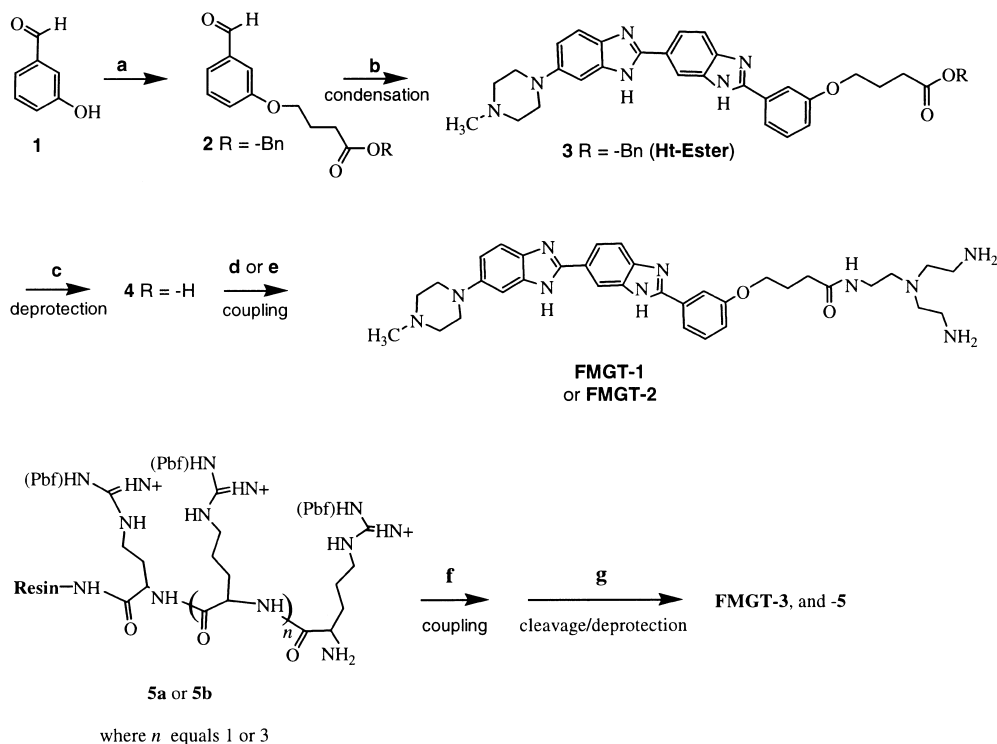
Scheme 1. (a) 4-Hydroxybutyrate, (\text{Ph})_3\text{P} , DEAD, DCM; (b) 2-(3,4-Diaminophenyl)-6-(4-methyl-1-piperazinyl)benzimidazole, nitrobenzene, 120^\circ\text{C} ; (c) \text{K}_2\text{CO}_3 , DMF, \text{H}_2\text{O} , 90^\circ\text{C} ; (d) PyBOP ® , tris(2-aminoethyl)amine, DMF; (e) PyBOP ® , spermine, DMF; (f) PyBOP ® , 4 , DMF; (g) 95% TFA, 2.5% triisopropylsilane, 2.5% water. Pbf = 2,2,4,6,7-pentamethyldihydrobenzofuran-5-sulfonyl.
